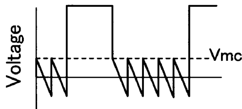
Sawtooth Wave 2
