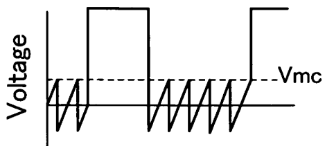
Sawtooth Wave 1
